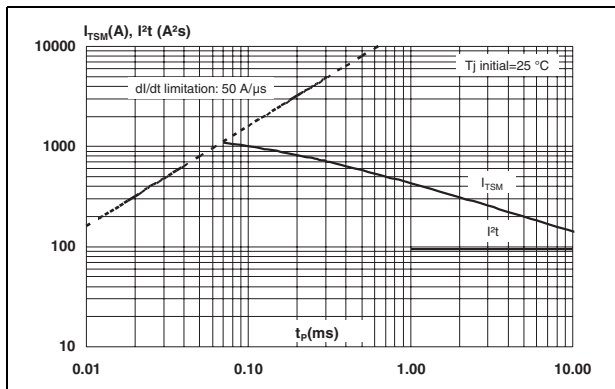
Figure 7. Non-repetitive surge peak on-state current for a sinusoidal pulse with width t_p < 10 ms and corresponding value of I²t
